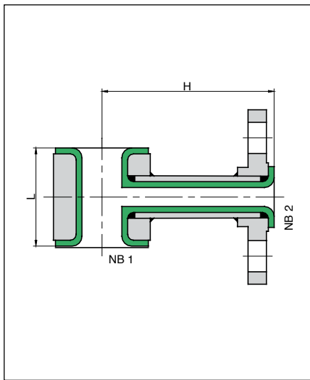
Instrument Tee, FF/LF
