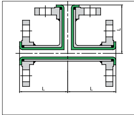
Equal Tee, FF
