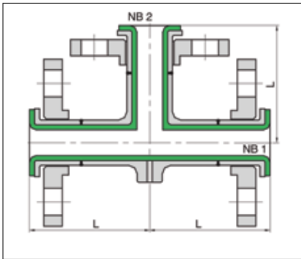
Steel Equal Tee, LF
