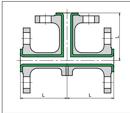
Cast Steel Equal Tee, FF
