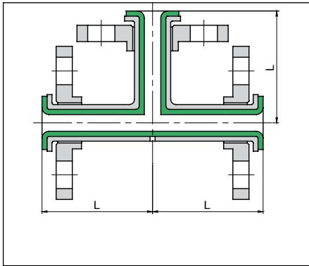
Stub-End Equal Tee, LF
