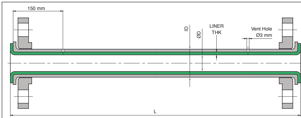
Stub-End Flange
