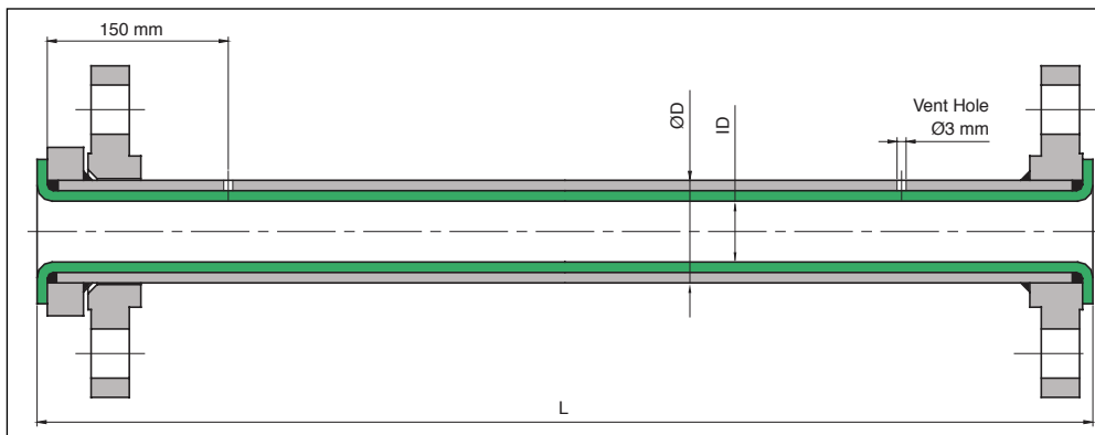
Fixed / Loose Flange
